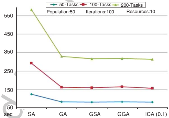
Fig. 13. Makespans for task variations with 100 iterations and 10 resources with a population of 50.
