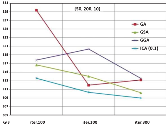
Fig. 10. Makespans for the state (50, 200, 10) for 100, 200, and 300 iterations.
