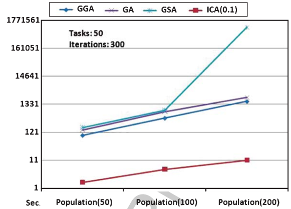
Fig. 12. Runtimes for 50 independent tasks with 300 iterations.
