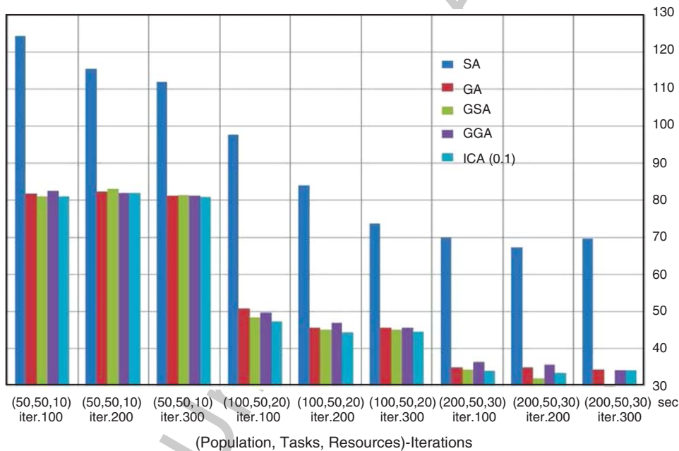
Fig. 9. Makespans for the different algorithms.
