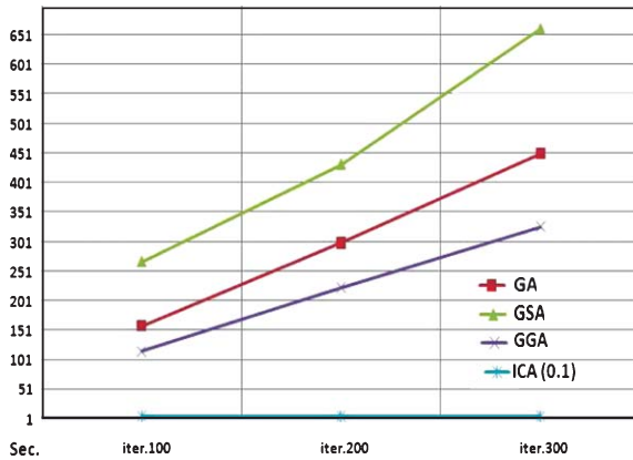
Fig. 11. Runtimes for the state (50, 200, 10) for 100, 200, and 300 iterations.
