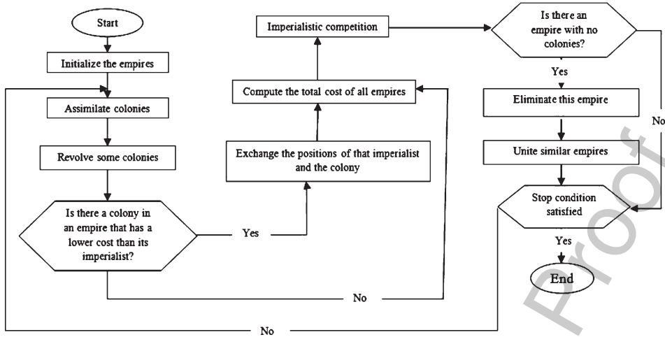
Fig. 2. ICA flowchart.
